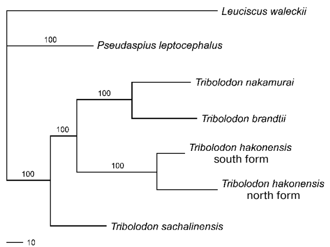
Fig. 2. Consensus tree ( L = 478 , CI = 0.76 , RI = 0.49 ) illustrating Cyprinid phylogenetic relationships with 1000 replicate bootstrap support.
